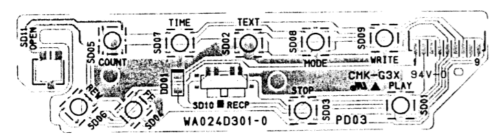
SWITCH P.C. BOARD (PD03)
