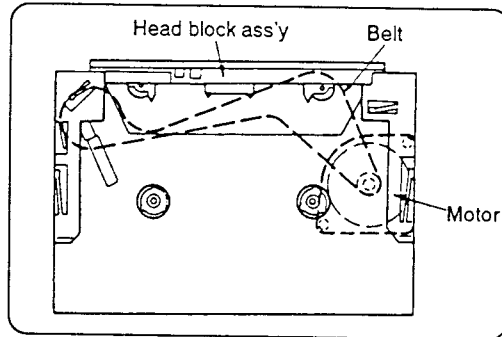
Mechanism to be repaired
