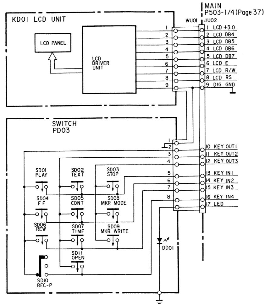
SWITCH P.C. BOARD (PD03)
