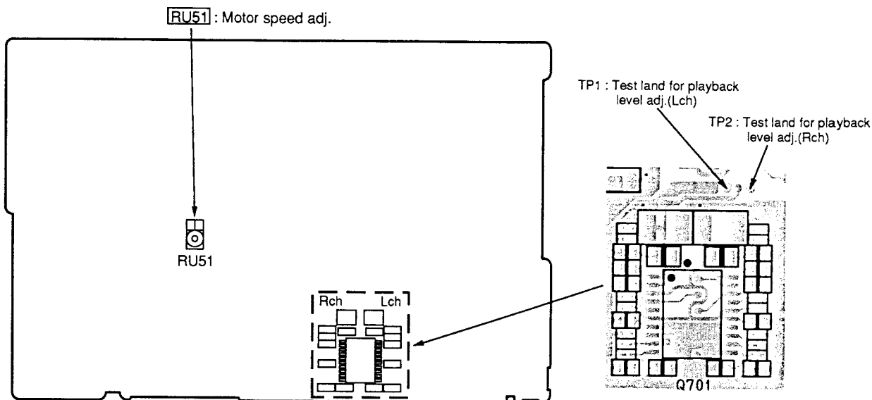
Fig. 1 MAIN PCB (P503)
